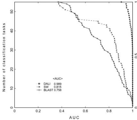
Figure 7: Database-wide comparison using cumulative AUC curves and similarity measures. The three methods are BLAST [20], Smith Waterman [21] and DALI [22], the comparison includes 55 classification tasks defined in the SCOP40mini dataset of the Protein Classification Benchmark [47]. The comparison was done by a nearest neighbor analysis using a groupwise scenario (Figure 7). Each graph plots the total number of classification tasks for which a given method exceeds a score threshold (left axis). The right axis shows the fraction of classification tasks (total number of tasks normalized to 1.00). The integral of the normalized cumulative AUC curve (which tends to the average of the constituent AUC values) is indicated for each method as \langle \text{AUC} \rangle .
